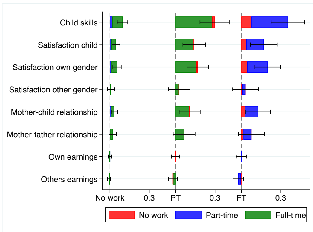
Figure A.17: Marginal effects – Alternative-specific variables (benchmark)
